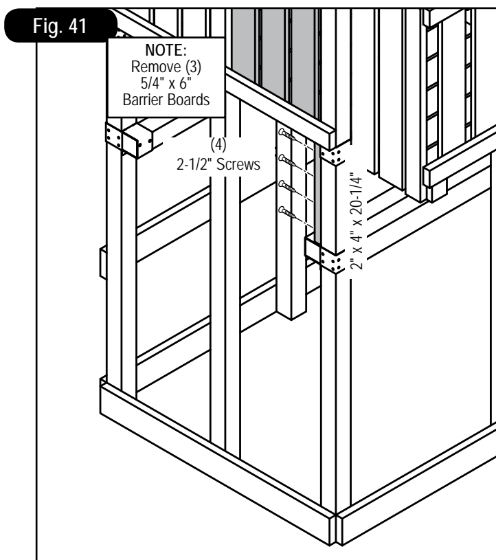
2-1/2" screw
