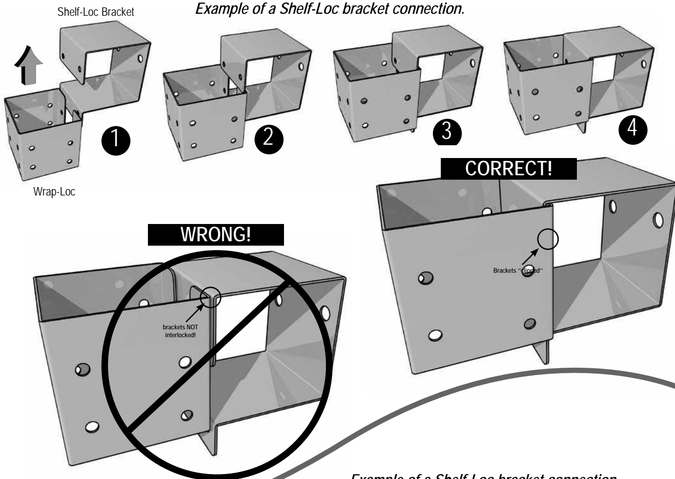
Example of a Shelf-Loc bracket connection.
